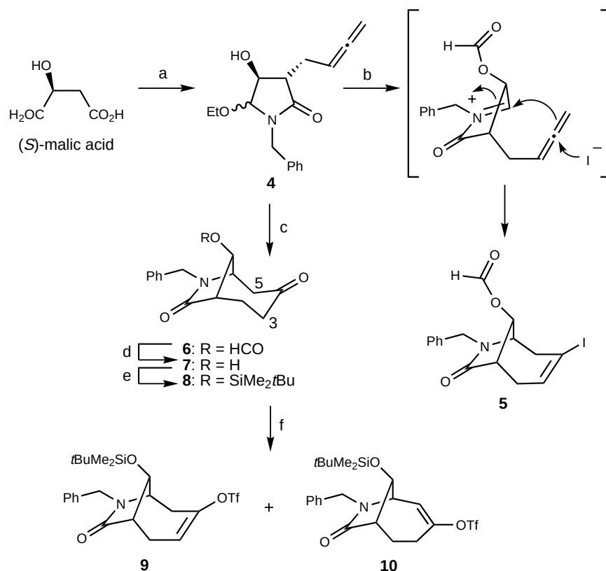
Scheme 1. Cyclization of 4 . a) Reference [11]; b) NaI (20 equiv), HCO 2 H (0.2 M), 85 °C, 18 h, 42 % of 5 + 34 % of 6 ; c) HCO 2 H, 85 °C, 18 h; d) satd NH 3 in MeOH, RT (room temperature), 15 min, 79 % over two steps; e) TBDMSCl (3 equiv), imidazole (4 equiv), DMAP (0.2 equiv), CH 2 Cl 2 , RT, 18 h, 96 %; f) LiHMDS (1.5 equiv), THF, –78 °C, 0.5 h, then PhNTf 2 (1.5 equiv), –78 °C → RT, 18 h, 45 % of 10 . DMAP = 4-(dimethylamino)pyridine, HMDS = hexamethyldisilazane, TBDMS = tert -butyldimethylsilyl, Tf = trifluoromethanesulfonyl.
